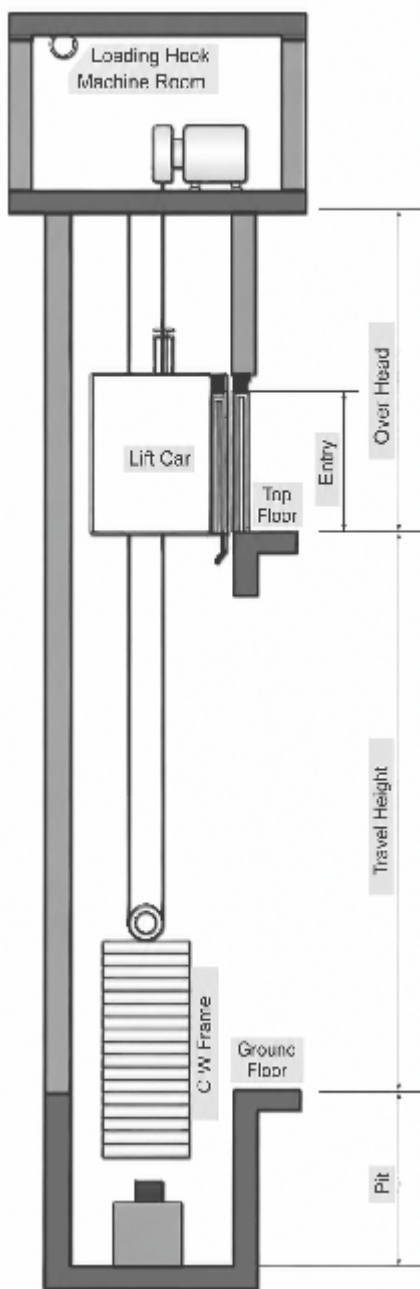
Hoistway Elevation Drawing
